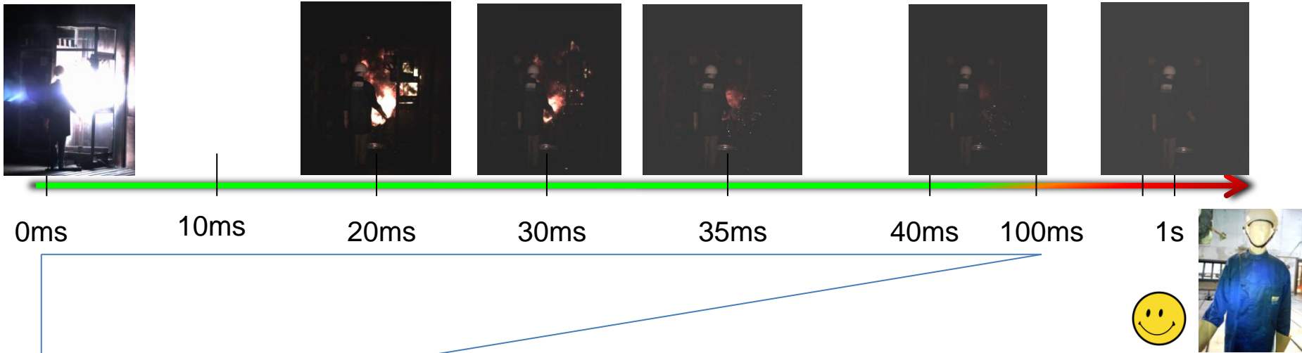
Arc fault inside conventional unit equipped with an ARC-KILLER SV-50E (16kA-1s)
